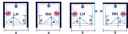
Bifold Door in Recess
