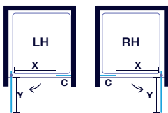
Pivot and Inline Door in Recess
